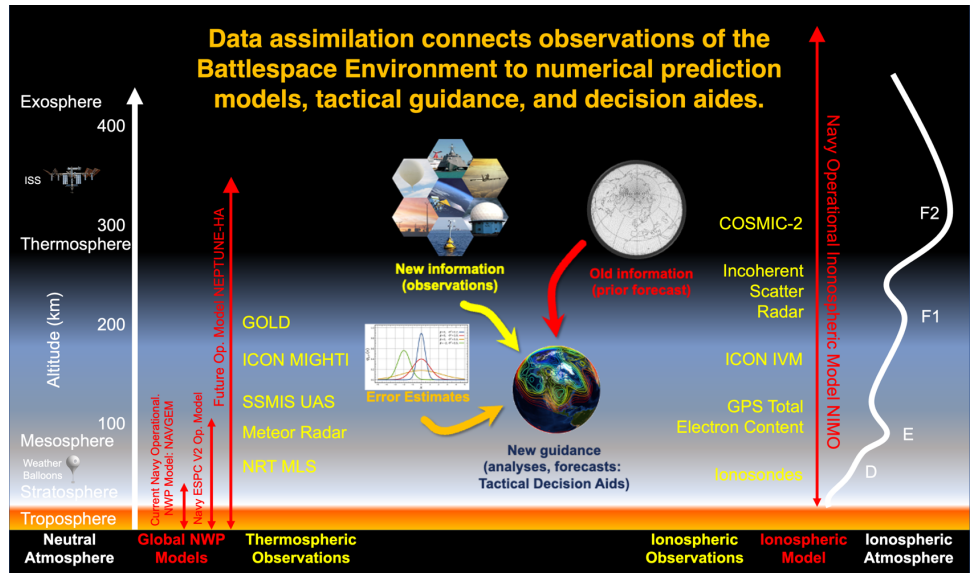
Operationalizing a Navy Coupled Upper Atmosphere Data Assimilation System
