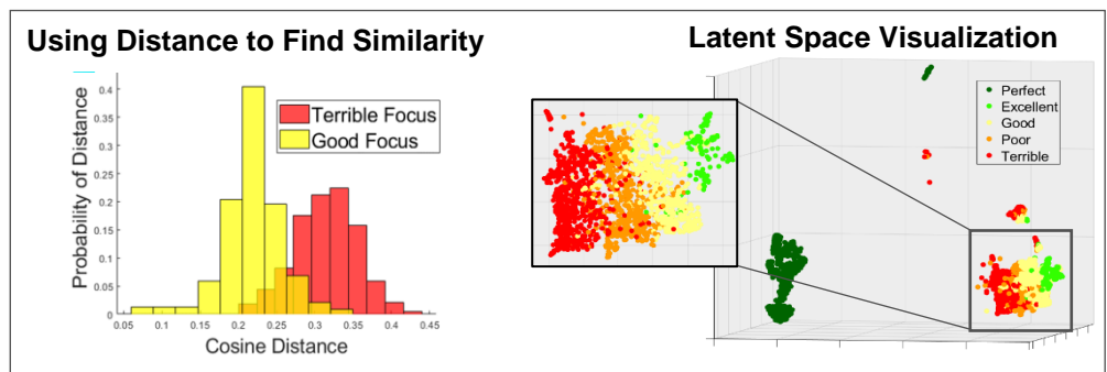
Latent space analysis to develop quantitative metrics for improved representation
