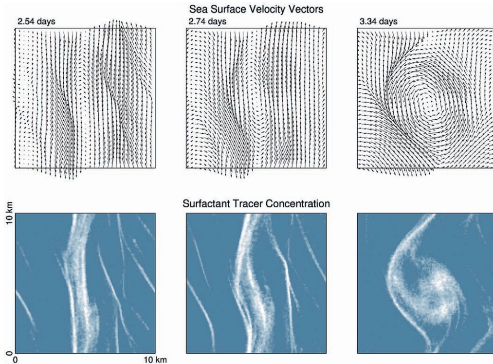
FIGURE 6 Plan view of the model sea surface. The longest velocity vector is 19.6 cm/s. The relative concentration of “surfactant” tracer is shown, with the upper 10% in white and lower 2% in blue.
