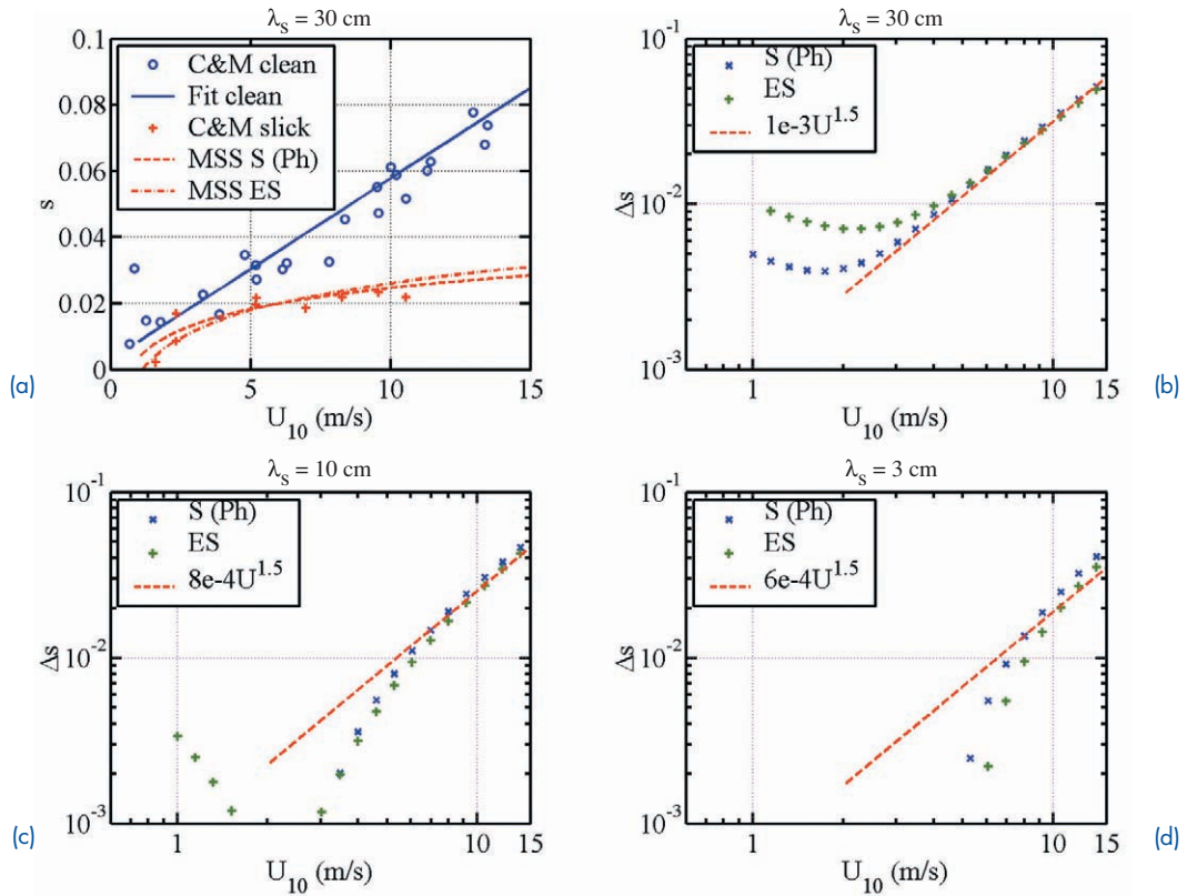
FIGURE 1 (a) The ocean surface roughness measured in clean and slick surface conditions (symbols) reported by Cox and Munk 2 and the comparison with calculated mean-square slopes based on established wave spectral models (curves). 1 (b)-(d) Breaking roughness calculated from the difference of the total roughness (clean water condition) and the mean-square slopes assuming three different cutoff wavenumbers.
