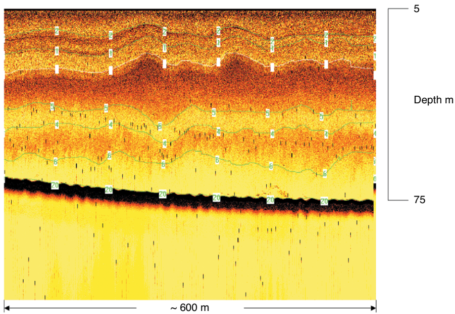
FIGURE 5 A 600-m flow visualization section showing the presence of a mode 2 internal wave on the New Jersey Shelf. The impact of mode 2 interfacial waves on the sound speed variability and acoustic signal variability is being addressed. Water depth is ~75 m.
