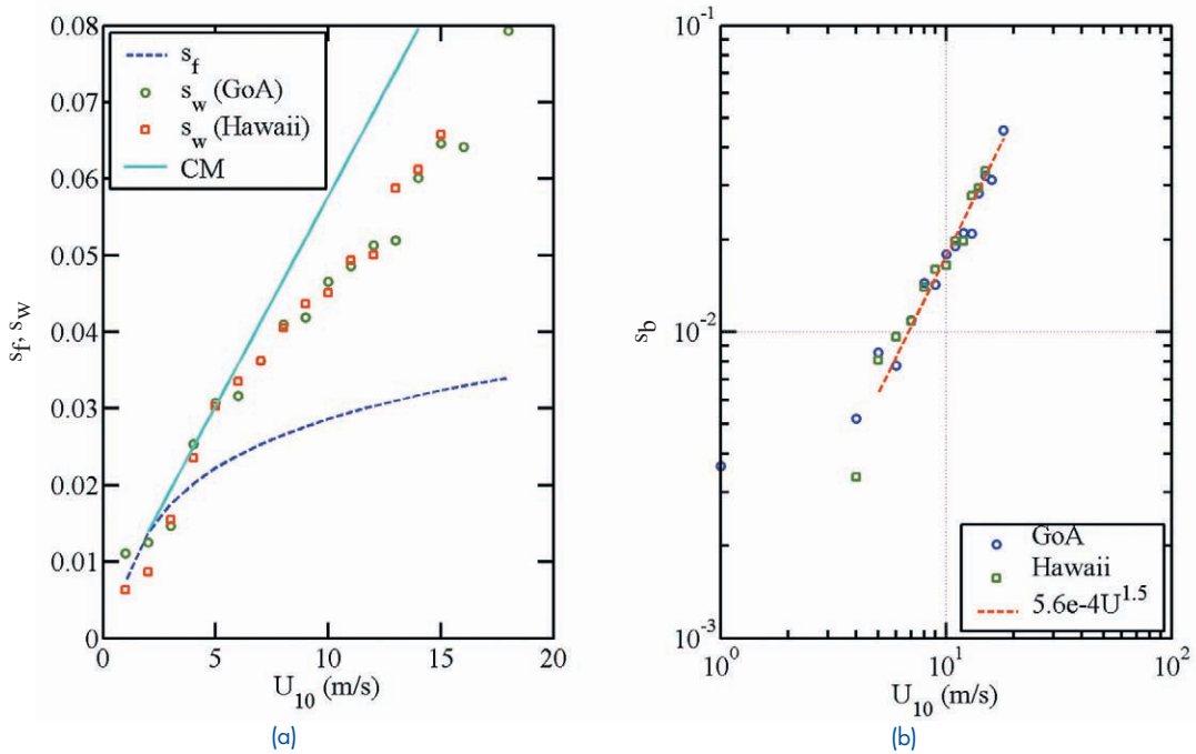
FIGURE 2 (a) Wind-induced roughness (symbols) derived from the TOPEX altimeter data. The calculated mean-square slope is shown with the dashed curve; for reference, the best-fit curve representing the CM clean water data is shown with the solid curve. (b) The breaking roughness derived from the altimeter data.
