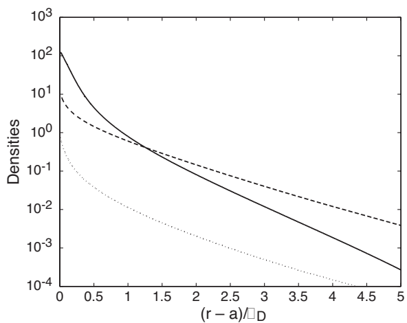
FIGURE 6 Trapped ion density (solid curve), deviation of untrapped ion density from ambient (dashed curve), and deviation of electron density from ambient (dotted curve). All densities are scaled to the ambient density n_0 . Note that the trapped ion density near the grain is 100 n_0 , and is ten times larger than the untrapped ion density.
