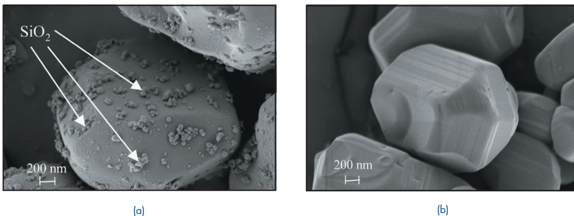
FIGURE 2 (a) Traditional “bucket chemistry” approach highlighting secondary phase particles of \text{SiO}_2 on \text{ZnS}:\text{Ag} phosphor particles, (b) a uniform and smooth coating of \text{SiO}_2 (10-nm-thick) on \text{ZnS}:\text{Ag} phosphor particles using the NRL-developed spray coating technique.
