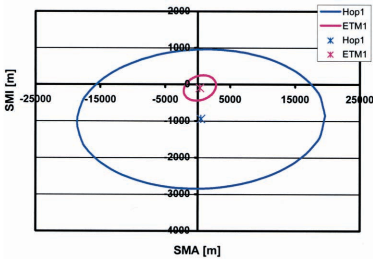
FIGURE 7(a) 95% EEP ellipse of SMA/SMI for medium elevation angle [ft].
