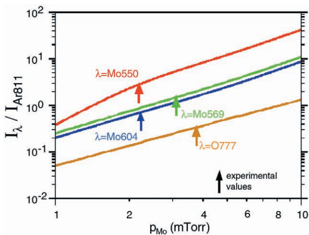
FIGURE 10 Ratio of line emission intensities from Mo and O with Ar as a function of the Mo partial pressure. Solid lines are from numerical simulations; the arrows indicate experimental values.
