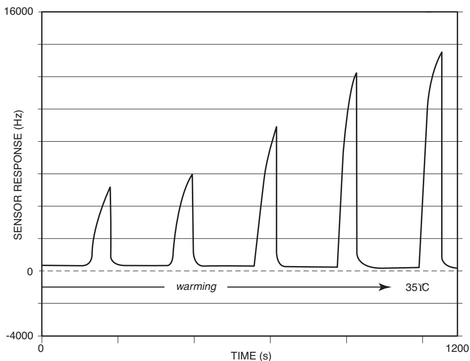
FIGURE 7 MIME sensor response to TNT vapor illustrating the increase in signal intensity as the TNT source is warmed from 25 to 35^{\circ}\text{C} during five purge-exposure cycles.
