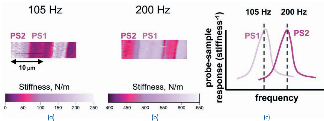
FIGURE 6 Stiffness images of alternating layers of polystyrene (PS) of two molecular weights at (a) 105 Hz and (b) 200 Hz. The contrast is due to frequency-dependent mechanical response of the polymers. The probe-sample response ( 1/\text{stiffness} ) as a function of frequency shown in (c) is consistent with the stiffness images.
