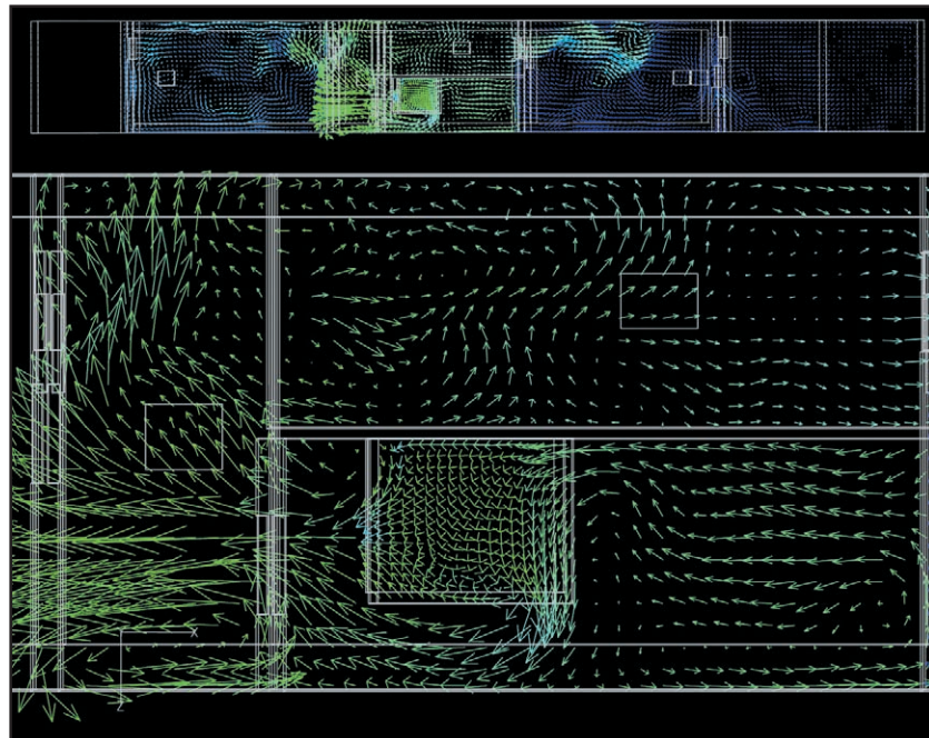
FIGURE 6 A detailed view using velocity vectors to illustrate the flow field in the laundry room and the adjacent passageway.
