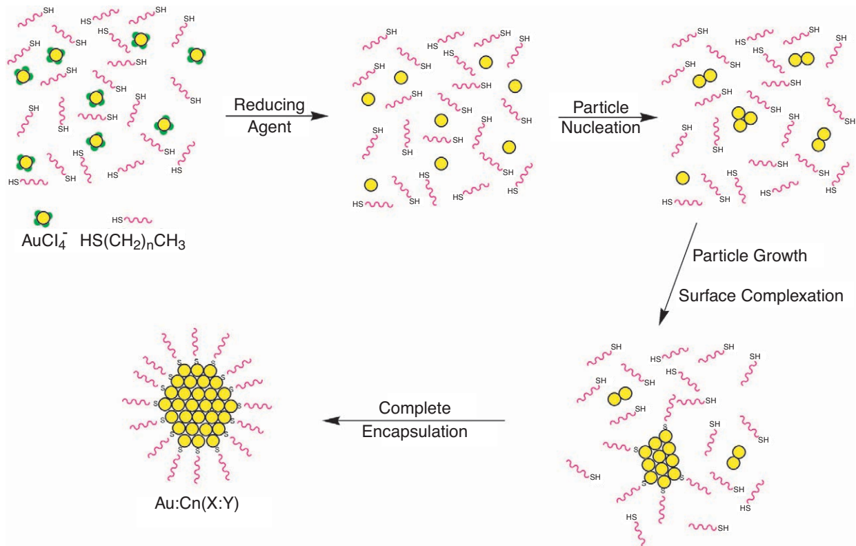
FIGURE 2 The alkanethiol stabilized cluster synthesis. After reduction of the gold ions, the competitive processes of gold particle growth and alkanethiol surface complexation determine the size of the gold nanocluster.
