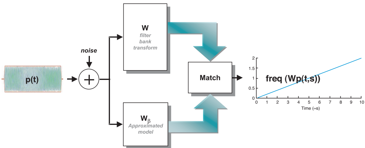
FIGURE 3 Estimation of signal IF via transform matching technique using a wavelet filter bank.
