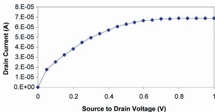
FIGURE 5 Typical current voltage (IV) trace for a device. This was obtained before streptavidin exposure, and the device has a dodecane thiol monolayer on the gate region.
