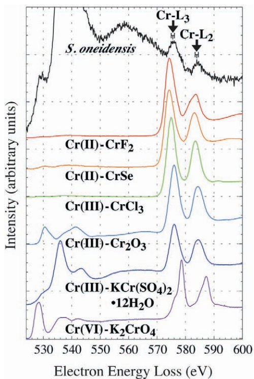
FIGURE 12 Comparison of EELS spectra of encrusted Shewanella oneidensis in the EC and Cr oxidation-state standards. Spectra were normalized to the intensity of the L 3 peak and offset from one another.
