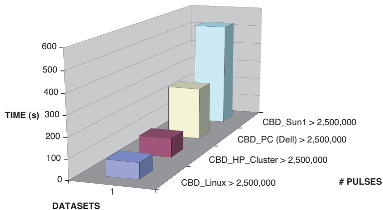
FIGURE 12 Evaluation of pruner processing time on four systems.
