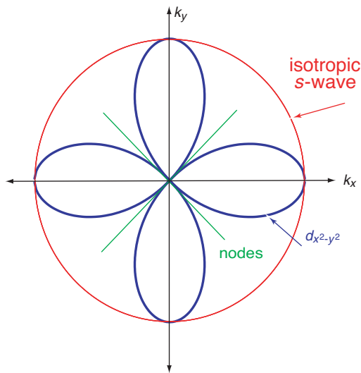
FIGURE 7 The superconducting pairing strength as a function of direction. The isotropic s -wave functional form (red) has no directional dependence. In contrast, the d_{x^2-y^2} functional form (blue) has directions of high and low pairing strength separated by 45 deg in 4-fold symmetry.
