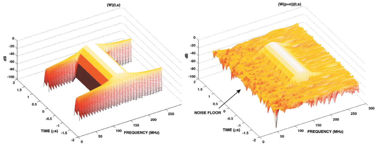
FIGURE 2 Time-frequency distributions associated with a fixed-frequency sinusoidal pulse: (left) distribution for signal only, and (right) distribution for signal plus noise.
