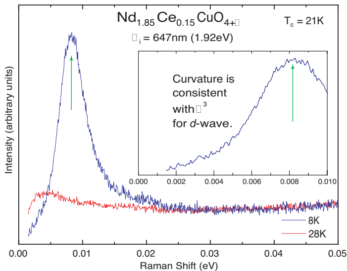
FIGURE 8 The Raman spectrum of \text{Nd}_{1.85}\text{Ce}_{0.15}\text{CuO}_{4+d} measured above and below the T_c of 21K. The incident laser energy of 1.92 eV is defined as zero, and only the downward “red” shift is plotted. The inset expands the low-frequency scale for the 8 K data to accentuate the curvature.
