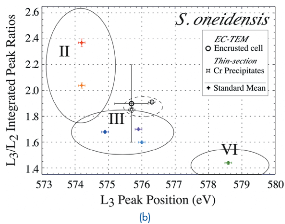
FIGURE 13 Correlation between measured L 3 /L 2 integrated-peak ratios and L 3 peak positions (a) Cr oxidation-state standards, (b) bacteria and precipitates (solid data points represent the mean of the data for a particular Cr standard).
