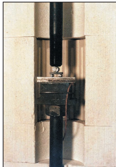
FIGURE 2 Elevated temperature short beam shear test for composite materials. This test evaluates the interlaminar shear strength of a composite and has become an important tool for studying the effects of cure cycle variations and environmental exposure on composite mechanical behavior.
