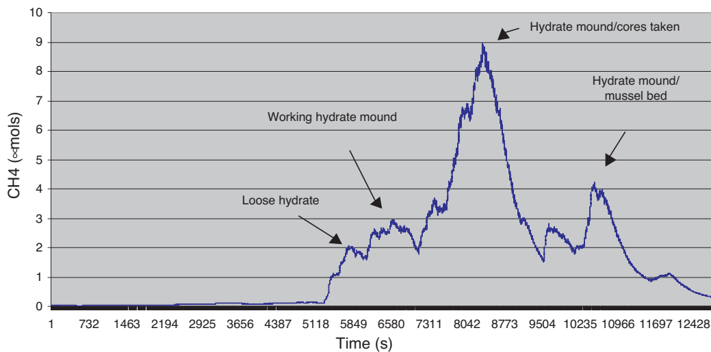
FIGURE 8 This plot shows that high methane concentrations can be observed with the methane sensor in the vicinity of hydrate outcroppings. Work was conducted on submarine dives in the Gulf of Mexico.
