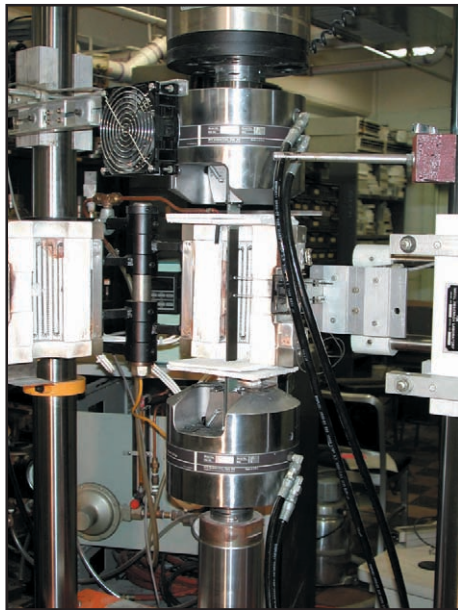
FIGURE 1 High-temperature polymer matrix composite tension test system developed at NRL. The system consists of a single-zone furnace mounted in a 500 kN capacity servohydraulic load frame. For applying force to the test specimen, 100 kN capacity side entry hydraulic grips are used.
