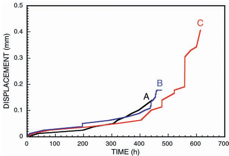
FIGURE 8 Time-displacement records for sustained load tension tests on a graphite-phthalonitrile unidirectional composite at 90% ultimate stress and 316 °C. There is very little deformation of the composite until after 400 h of exposure. Failure of the material occurred at exposure times of between 443 (A) and 614 (C) h.
