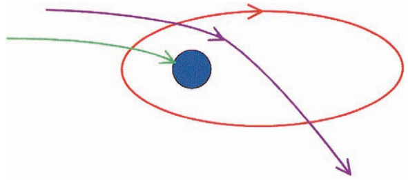
FIGURE 5 According to orbital-motion-limited theory, ions fly in from the ambient plasma and either miss the grain and fly back out to the ambient plasma (purple orbit), or hit the grain and stick (green orbit). Our theory also includes trapped ions (red orbit) created by collisions.
