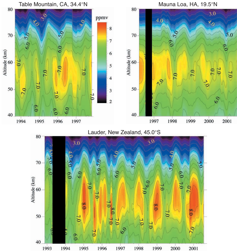
FIGURE 2 Full data record from the three sites where WVMS instruments have been deployed. Note the seasonal cycles at all three sites. Because the Lauder, NZ, site is farthest from the equator, it shows the most pronounced annual variation.
