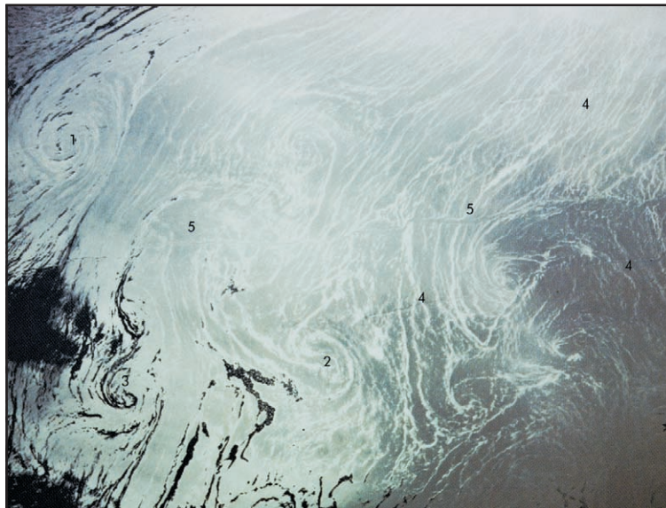
FIGURE 4 Sun-glint photograph of the central Mediterranean Sea taken from the Space Shuttle in 1984. Area covered (cropped from the original published photo) is ~150 km on each side. The bright bands are naturally occurring slicks. Numbers 1, 2, and 3 identify three of the several spirals visible on the sea surface. Some ship wakes are also visible on the surface and are indicated by numbers 4 and 5. (Courtesy of National Aeronautics and Space Administration, Oceanography from Space , 1986)
