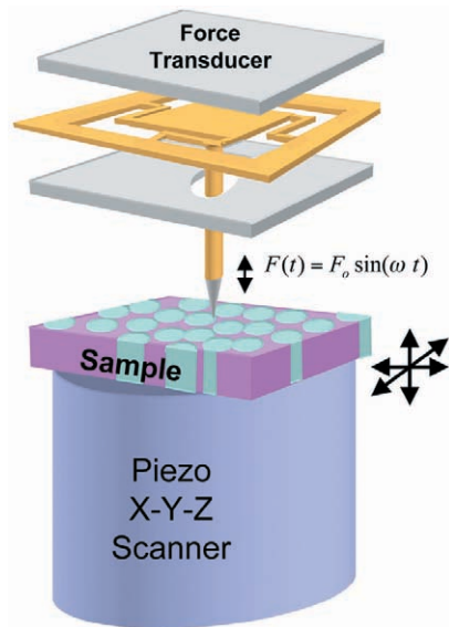
FIGURE 4 “Hybrid” scanning nanoindenter. The load-displacement response of a probe attached to a movable plate is actuated electrostatically to apply force; the displacement response is monitored by capacitive techniques. Sample x-y positioning and scanning are accomplished through a piezo-tube scanner.
