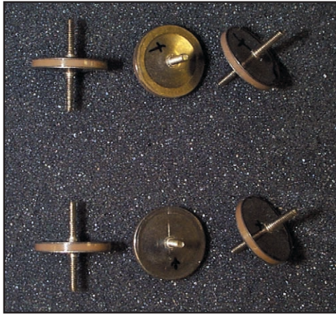
FIGURE 9 The cymbal flextensional electromechanical driver.
