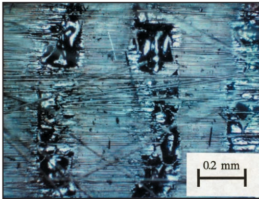
FIGURE 7 Surface condition of a graphite-phthalonitrile composite after exposure to 538 °C for 400 s where the graphite fibers are exposed from a loss of the phthalonitrile resin due to oxidation
