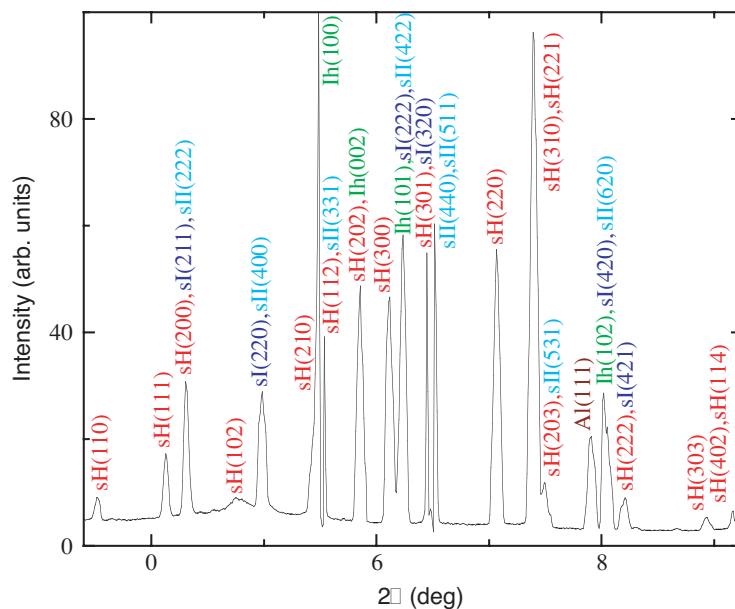
FIGURE 10 X-ray diffraction of natural hydrate collected from the Gulf of Mexico. Measurement performed at 500 psi and 150 K using 33 keV (0.3757 Å) photons from the Advanced Photon Source. Diffraction peaks labeled from hydrate structure H (red), structure I (blue), and structure II (cyan), and water ice Ih (green).
