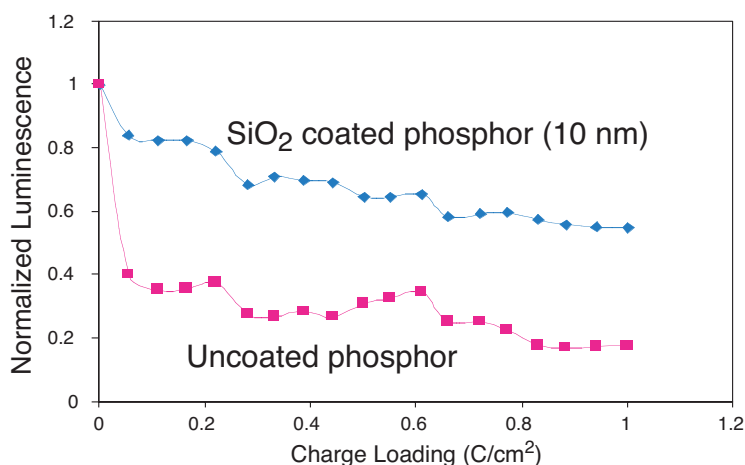
FIGURE 3 Normalized aging curves for coated and uncoated \text{ZnS}:\text{Ag} phosphor.
