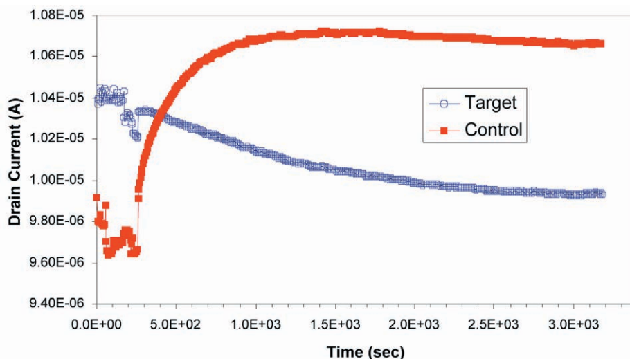
FIGURE 6 Continuous monitoring of drain current from four devices (averaged) at 0.5 V drain-source bias during exposure to complement DNA solution (target) and pure buffer solution (control). Initially, neither solution had DNA. The cover was removed from these photosensitive devices at about 50 s, and a quantity of buffer was withdrawn and replaced with target DNA solution in the target cell at approx. 200 s. The cover was then replaced at 280 s, leading to the abrupt jump in both signals simultaneously. These data illustrate the importance of both baselines and control devices.
