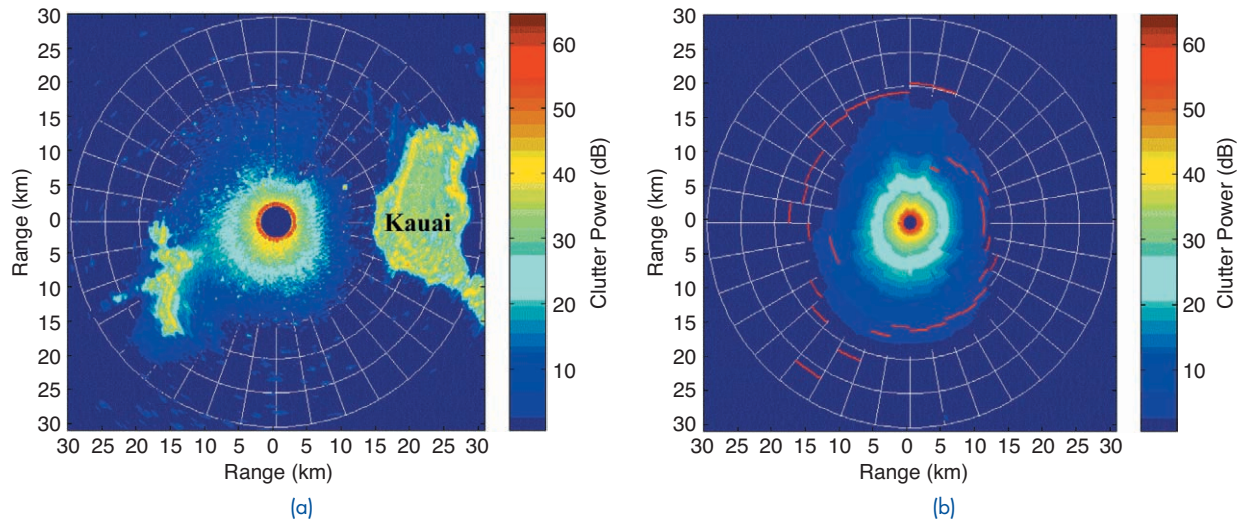
FIGURE 5 (a) Observed clutter map from the USS O'Kane radar on 3 December 1999 with islands of Kauai and Niihau; (b) modeled clutter map computed from linkage of diverse model systems described in text.
