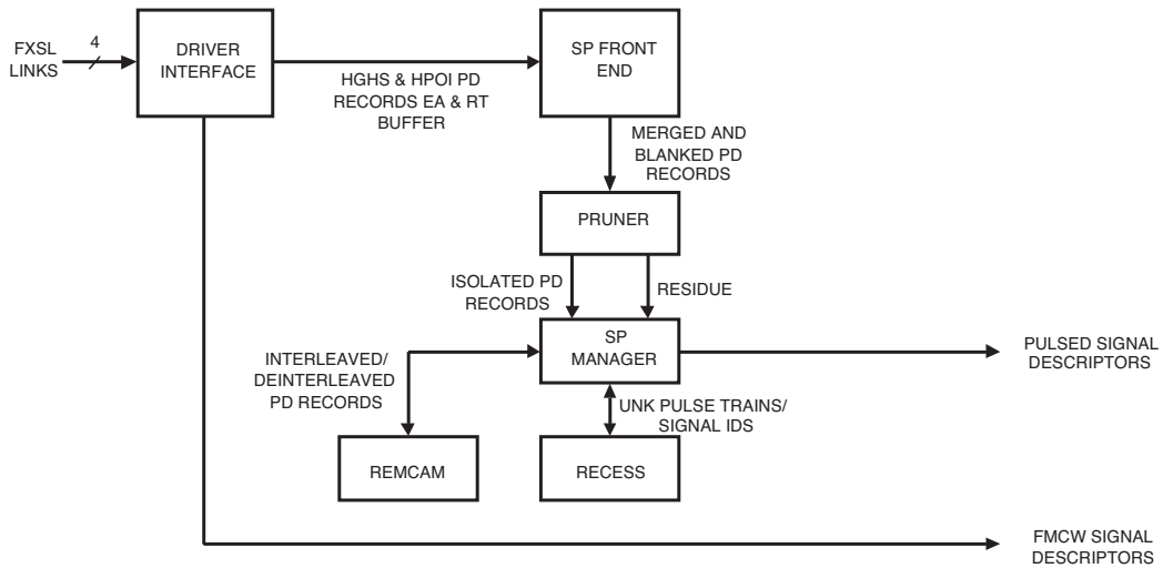
FIGURE 11 Signal processing signal flow.
