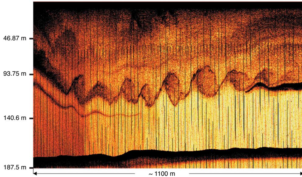
FIGURE 6 An 1100-m flow visualization record of a series of shear instabilities associated with the first lobe of a Luzon Basin soliton. Water between two layers is being mixed by roughly 40-m amplitude shear instabilities. This will cause short acoustic coherence lengths.
