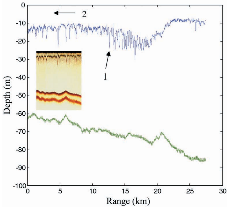
FIGURE 4 The range variability of the depth of an isosound speed layer (blue line) shows both long wavelength and short wavelength features. The ocean bottom is the green line. The direction of propagation of the internal tide, the 20-km depression feature, is shown by arrow 2. The insert shows a section of the acoustic flow visualization data that was digitized to obtain the 27-km realization of the sound speed variability. The vertical displacement of the mixed layer by the internal wave field is clear. The ocean bottom reflection is the upper red reflection. The lower bottom red reflection is an artifact. (From Fig. 24 of Ref. 1.)
