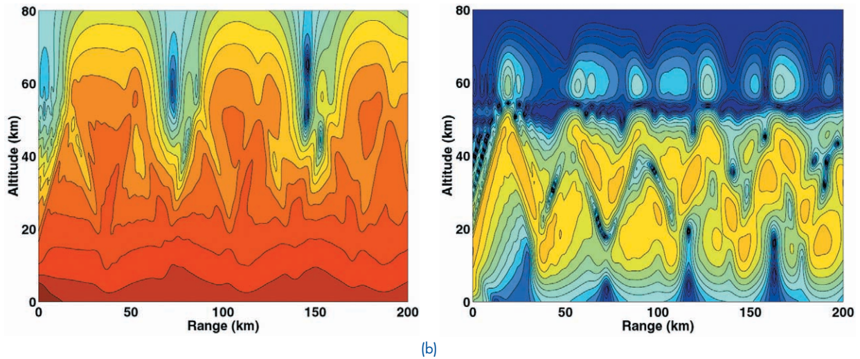
FIGURE 1 (a) Model atmospheric profiles for density, sound speed, and buoyancy frequency obtained by smoothing tabulated standard atmospheric profiles. (b) Intensity plots of 3-MHz (left) AG and (right) pure gravity waves. The AG wave contains a large amount of energy near the ground due to a contribution of the Lamb wave; dynamic range of the plots is 50 dB.
