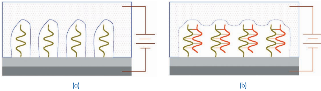
FIGURE 1 (a) Thin insulating film modified with single stranded DNA and in contact with a conducting solution on one side and a conducting layer on the other. An electrode immersed in the solution establishes the solution potential with respect to the conducting substrate. The capacitance between the solution and the substrate is a combination of the insulating film, the DNA molecules, and the double layer at the liquid-insulator interface. (b) The same system after hybridization. The bound pair displaces substantial fluid from the insulating film, decreasing the system capacitance.
