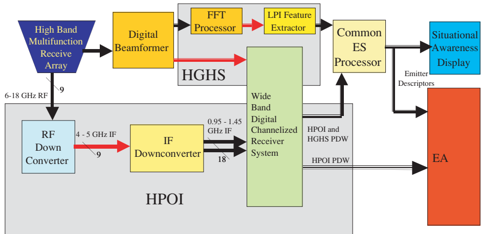
FIGURE 10 Electronic surveillance functions in AMRFC.
