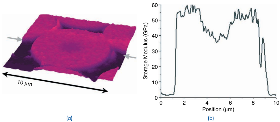
FIGURE 5 (a) Two-dimensional map of the elastic modulus of a carbon fiber-epoxy composite material. Brighter regions of the image correspond to higher modulus. (b) Cross-section line scan through the center of the image (marked by arrows in (a)) shows the storage modulus in the epoxy and the modulus gradient at the center of the fiber.
