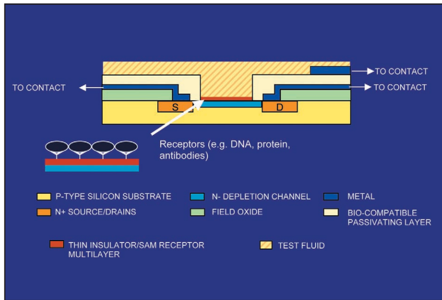
FIGURE 2 Schematic illustrating construction of the device. Except for the absence of the traditional gate electrode overlaying the channel, it is a typical depletion mode n -channel insulating gate field effect transistor.
