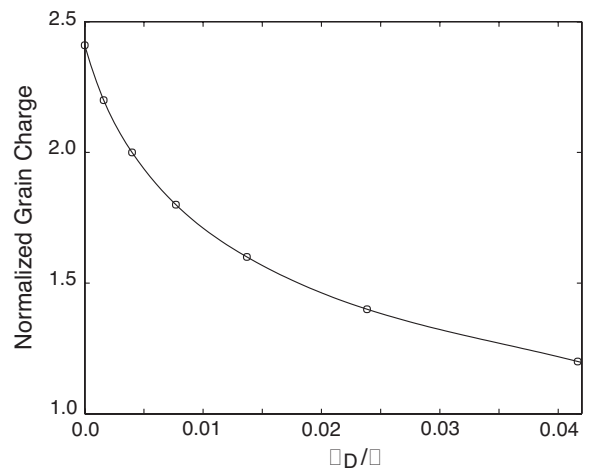
FIGURE 7 Grain charge (in normalized units) as a function of \lambda_D/\lambda , where \lambda is the mean free path and \lambda_D is the Debye screening length.
