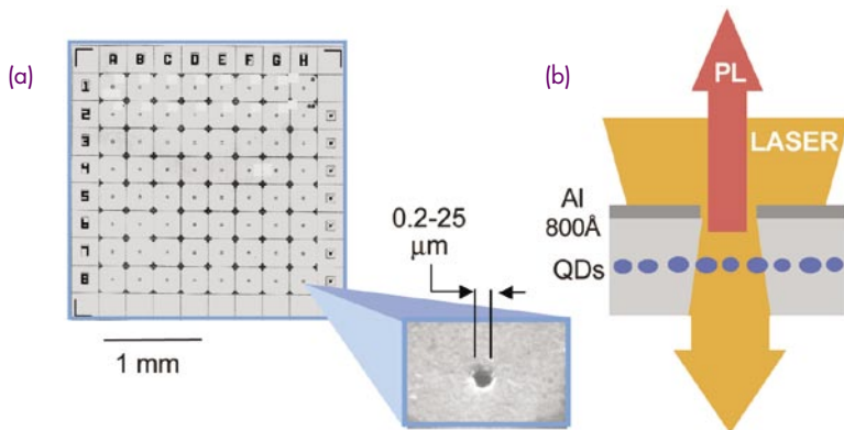
FIGURE 4 (a) Image of an aluminum aperture mask on a GaAs QD sample used for single QD spectroscopy. (b) Cross-sectional schematic of laser excitation and PL of a small number of QDs through a submicron aperture.
