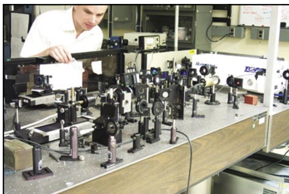
Femtosecond laser system for ultrafast dynamics; nonlinear mixing techniques are used to generate femtosecond pulses over a wide range of wavelengths. These techniques include photochemistry and vibrational energy dynamics of ions in solution and in reverse micelles.
