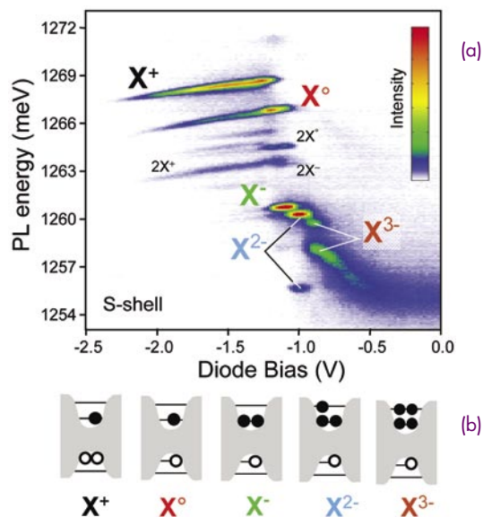
FIGURE 5 (a) PL intensity map as a function of PL energy and diode bias. PL features from various charge states of excitons ( X symbols) and biexcitons ( 2X symbols) are labeled accordingly. (b) Electron and hole configurations for the various excitons as labeled in (a).
