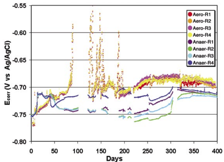
FIGURE 11 Average E_{\text{corr}} (vs Ag/AgCl) over time values for C1020 samples in stagnant aerobic (aero) and anaerobic (anaer) conditions displayed by row (R). R1, R2, R3 – vertically orientated samples, with R1 being at the top of the tank, R3 toward the bottom, and R2 between the two. R4 – horizontally orientated sample at the bottom of the tank.
