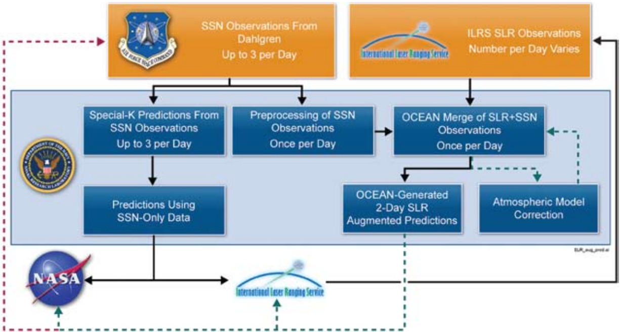
FIGURE 6 The data flow and processing of ANDE observations. The green dashed lines represent functions demonstrated during the ANDERR mission. The red dashed line is expected to be complete after the final ANDE flight.
