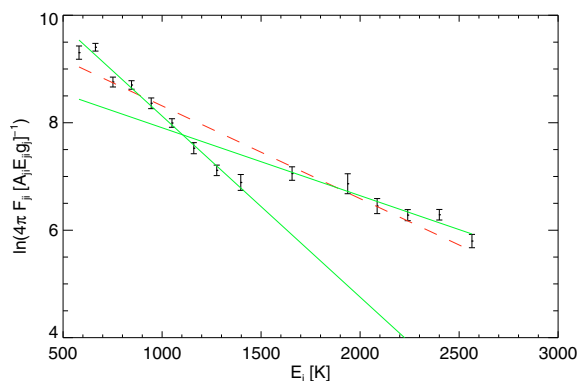
Fig. 5. Rotational diagram of the CO lines in HD 100546 (crosses), overplotted with our models, using Eq. (2) from Justtanont et al. (2000) . A single temperature fit (dashed) gives reasonable results, but a two-temperature approach (solid) yields a better description of the data. CO J = 23-22 and J = 31-30 are blended with H 2 O and OH respectively and were not used in the fit, nor are they shown here.
