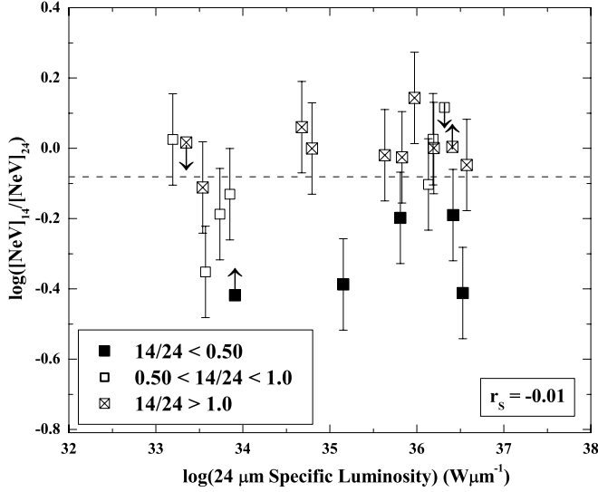
FIG. 5.—Observed [\text{Ne v}] line ratio as a function of the 24\ \mu\text{m} specific luminosity for our sample of galaxies. The error bars shown here represent the calibration uncertainties on the [\text{Ne v}] line flux ratio as in Fig. 3. The symbol type indicates the 14\ \mu\text{m}/24\ \mu\text{m} continuum ratio.
