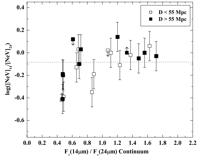
FIG. 6.— [\text{Ne v}] line ratio vs. the F_{\nu}(14\ \mu\text{m})/F_{\nu}(24\ \mu\text{m}) continuum ratio for our sample. In both plots, the error bars mark the calibration uncertainties on the line ratio. There is a correlation between the line and continuum ratios which suggests that extinction affects the observed line flux ratios. Top : The majority of galaxies with ratios below the LDL are type 2 objects, implying that the extinction toward the [\text{Ne v}] -emitting region may be due to the torus. Bottom : The correlation shown here is not an artifact of aperture variations between the SH and LH slits. The correlation holds when only the most distant galaxies are considered.
