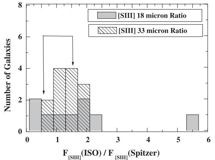
FIG. 10.—Ratios of the [S III] flux from ISO and Spitzer for the 18 and 33 \mu\text{m} lines. The range indicated with arrows is that corresponding to the absolute flux calibration for ISO (20%) and Spitzer (15%). The [S III] emission is indeed extended beyond the Spitzer slit for many galaxies, suggesting that the [S III] emission may be produced in star-forming regions. We note that IRAS 20551 and IRAS 23128 are point sources with Spitzer 18 \mu\text{m} fluxes greater than the ISO fluxes from Genzel et al. 1998; however, they fall within the Genzel et al. (1998) quoted errors of 30% and the Spitzer calibration error of 15%. Galaxies with fluxes from Dale et al. 2006 are not included in this plot since the extraction aperture for these galaxies is comparable to the 18 \mu\text{m} ISO slit.
