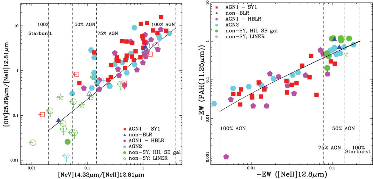
Figure 3. Left panel: [\text{O IV}]25.9 \mu\text{m}/[\text{Ne II}]12.8 \mu\text{m} line ratio versus [\text{Ne V}]14.3 \mu\text{m}/[\text{Ne II}]12.8 \mu\text{m} line ratio. Both axes correlate with the strength of the AGN. The black line shows the behaviour of the analytical model (Tommasin et al. 2010). Right panel: [\text{Ne II}]12.8 \mu\text{m} equivalent width versus PAH 11.25 \mu\text{m} equivalent width. Both quantities in this plot correlate with the strength of the star-formation component in each galaxy. The black line shows the behaviour of the analytical model (Tommasin et al. 2010).
